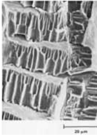
Fig. 39 Flutes and cleavage from SCC of \beta -annealed Ti-8Al-1Mo-1V in methanol. Source: Ref 89
