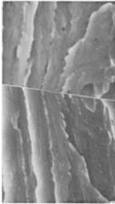
Fig. 645 Hydrogen embrittlement of AISI type 304 tested under constant load in pure hydrogen gas at 100 kPa (1 atm) and 25 °C (75 °F). The two-part fractograph compares matching fracture surfaces. Note the quasi-cleavage-type facets. They generally exhibit more ductility (have a rougher surface) than classic cleavage facets. See also Fig. 629. SEM, 6000× (R. Liu, N. Narita, C. Altstetter, H. Burnbaum, and N. Pugh, University of Illinois)
