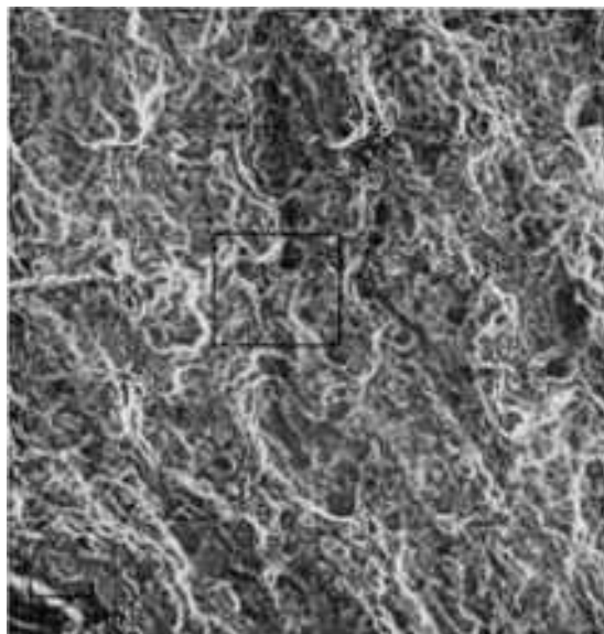
Fig. 1030 Highly magnified view of fatigue striations typical of those in areas A in Fig. 1027. In general, these striations were parallel with the flaw B-B. Dimples characterized the remainder of the fracture. Inclusions near the flaw suggested that it was the result of a pipe not cropped from the ingot. SEM, 3000×
