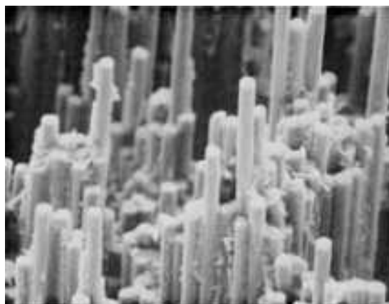
Fig. 1303 A typical area in the tensile failure region of the carbon/epoxy flexural specimen shown in Fig. 1300 and 1301. Note the long, protruding fibers with some attached epoxy remaining. This area resembles typical regions in a specimen failed in pure tension. See also Fig. 1302. SEM (same conditions as in Fig. 1294), 500× (The composite specimens shown in Fig. 1296, 1297, 1298, 1299, 1300, 1301, 1302, 1303, 1304, 1305, 1306, 1307, 1308, 1309, and 1310 all consisted of circa 1978 Thornel 300 fibers in Narmco 5208 epoxy resin. The composites were all fabricated by lay-up of prepreg tape and were autoclave cured 175 °C (350 °F) according to the manufacturer's recommendations. Specimens were then end-tabbed and cut in accordance with the
