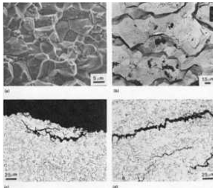
Fig. 100 Fracture in a thermally embrittled cobalt-free high-titanium maraging steel. (a) Secondary electron image of fracture surface, 1300 ×. (b) TEM extraction fractograph, 2150 ×. (c) Light micrograph of fracture edge, 260 ×. (d) Light micrograph of internal cracks, 260 ×. Light micrograph specimens etched with modified Fry's reagent
