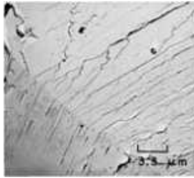
Fig. 28 Cleavage fracture in Armco iron broken at -196 °C (-321 °F), showing river patterns, tongues, and (from bottom right to top left) a grain boundary. TEM p-c replica, 3000×
