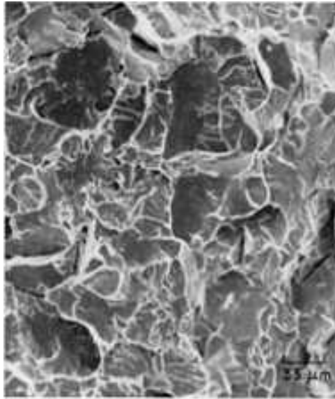
Fig. 1208 This SEM fractograph of the unaged specimen in Fig. 1207 shows quasi-cleavage facets. The impact energy was less than 27 J (20 ft · lb). 300× (Figures 1207, 1208, 1209, 1210, 1211, 1212, 1213, 1214, 1215, 1216, 1217, and 1218 present six related pairs of light and SEM fractographs of specimens of an Fe-12Ni-0.5Ti alloy intended for use at cryogenic temperatures. The series shows the effect on Charpy impact energy at -196 °C (-321 °F), and on fracture-surface characteristics, of the temperature of aging after austenitizing at 900 °C (1650 °F) for 2 h and air cooling.)
