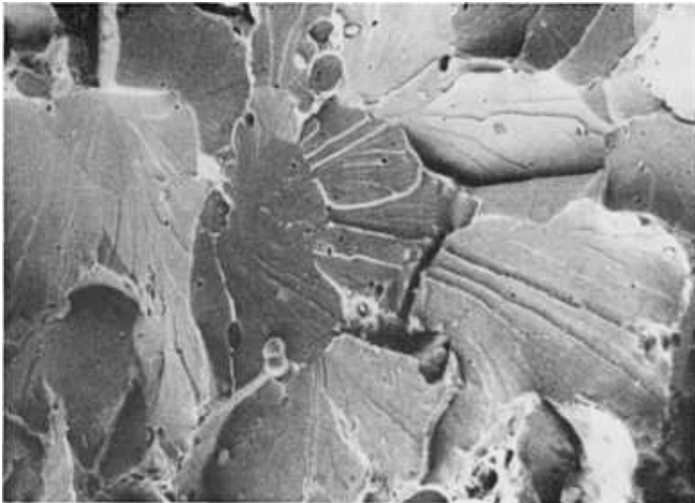
Fig. 119 Brittle fracture of AISI 1020 hydraulic jack shaft. Failure originated at root of machined thread. Corrosion (evident on part) and fatigue (due to repeated loading of shaft) may also have played roles in the failure. Photomicrograph of fracture surface shows transgranular cleavage with individual grains identified by changes in fracture plane orientation. The apparent grain size of 100 to 125 \mu\text{m} corresponds to a ductile-to-brittle transition temperature of approximately 100 °C (212 °F). SEM, 450× (J.M. Rigsbee, University of Illinois)
