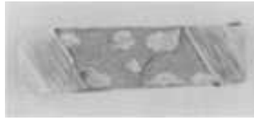
Fig. 80 Example of the macroscopic appearance of hydrogen flakes in plate steel. 1.6 ×
