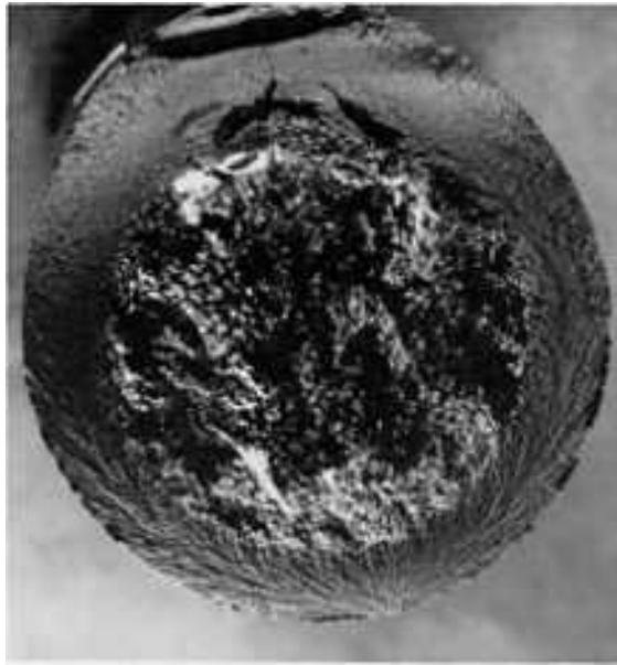
Fig. 220 Fracture surface of the modified SAE 1050 axle shaft shown in Fig. 221. Note chevrons pointing to fracture origin in the fine structured case. See also Fig. 222, 223, 224, 225, 226, and 227. 2.75×
