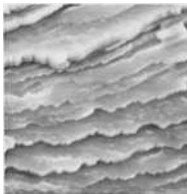
Fig. 629 Stress-corrosion cracking facets on the fracture surface of an AISI type 304 sample tested under constant load in \text{MgCl}_2 solution at 155 °C (310 °F). The steplike features are analogous to cleavage facets. See also Fig. 645. SEM, 3000× (R. Liu, N. Narita, C. Altstetter, H. Birnbaum, and N. Pugh, University of Illinois)
