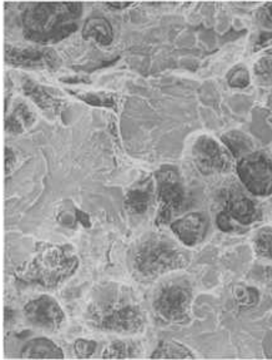
Fig. 92 Fracture surface of a ferritic-pearlitic ductile iron. Note ductile fracture of ferrite in matrix around nodules and cleavage (brittle) fracture of pearlite in matrix. SEM, 50× (W.L. Bradley, Texas A&M University)
