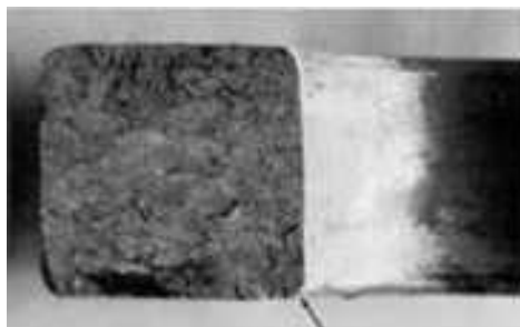
Fig. 1079 Fracture surface outboard of the bolthole in the clevis-attachment lug at right in Fig. 1078. Entire surface is typical of stress-corrosion cracking. Origin is at arrow (lower right corner of surface). 4×
