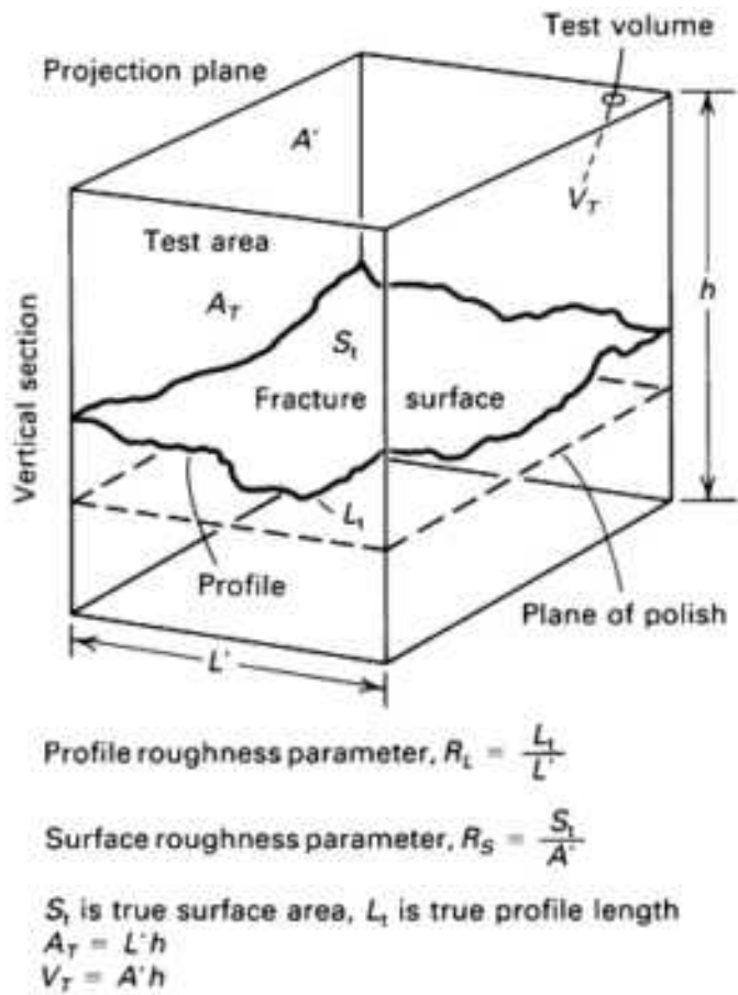
Fig. 10 Arbitrary test volume enclosing a fracture surface
