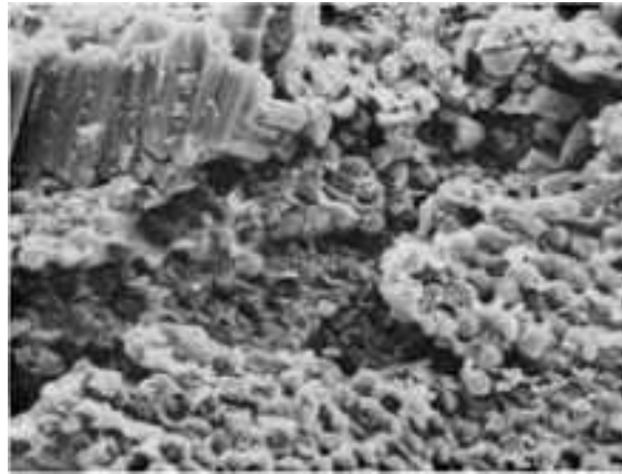
Fig. 1302 Another view of the carbon/epoxy flexural specimen shown in Fig. 1300 and 1301. This fractograph shows a typical area in the compressive failure region at a higher magnification. Note the crushed and crumpled fibers. See also Fig. 1303. SEM (same conditions as in Fig. 1294), 500× (The composite specimens shown in Fig. 1296, 1297, 1298, 1299, 1300, 1301, 1302, 1303, 1304, 1305, 1306, 1307, 1308, 1309, and 1310 all consisted of circa 1978 Thornel 300 fibers in Narmco 5208 epoxy resin. The composites were all fabricated by lay-up of prepreg tape and were autoclave cured 175 °C (350 °F) according to the manufacturer's recommendations. Specimens were then end-tabbed and cut in accordance with the ASTM D3039. The 0° and 90° tensile specimens were tested in accordance with ASTM D3039, and the 0° flexural three-point-bend specimens were tested in accordance with ASTM D790. The composites were dried before testing in the same manner as the epoxy specimens described in Fig. 1294 and 1295. "Dry" specimens were tested as-dried and had essentially 0 wt% moisture. "Room" moisture specimens had about 0.6 wt% moisture, having been placed after drying in a chamber at 60 °C (140 °F) and 60% relative humidity for at least 2 months and then placed in a drawer in the laboratory for several months before testing. "Wet" specimens had about 1.5 to 2.0 wt% moisture, having been placed for several months in an environmental chamber at 60 °C (140 °F) and 100% relative humidity. The composites were tested at moisture conditions designed not to alter their conditioning, and at the temperatures noted.) (L. Clements, San Jose State University, and J.C. Liu, Cornell University)
