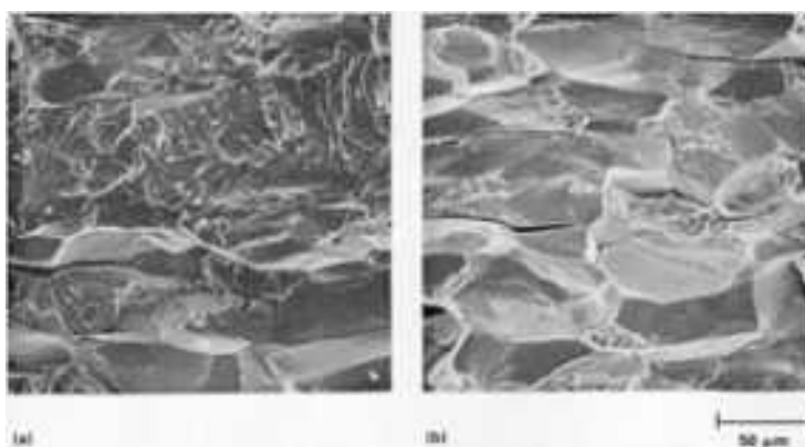
Fig. 51 Stress-corrosion fractures in a 25% cold-worked type 316 austenitic stainless steel tested in a boiling ( 154^\circ\text{C} , or 309^\circ\text{F} ) aqueous 44.7% magnesium chloride solution. At low ( 14 \text{ MPa } \sqrt{m} , or 12.5 \text{ ksi } \sqrt{in.} ) K_I values, the fracture exhibits a combination of cleavage and intergranular decohesion (a). At higher ( 33 \text{ MPa } \sqrt{m} , or 30 \text{ ksi } \sqrt{in.} ) values of K_I the principal mode of fracture is intergranular decohesion (b). Source: Ref 181
