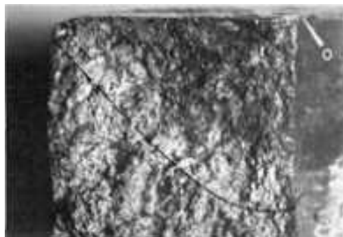
Fig. 934 Enlarged view of one fracture surface of the lug in Fig. 933, more clearly showing the fatigue-crack region at top left corner of the bore. Crack was nucleated at corner marked by arrow at "O." Fatigue area extended approximately to dashed line. See also Fig. 935 and 936. 8×
