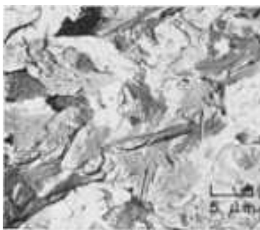
Fig. 462 Surface of a tension-overload fracture in a notched specimen of the same AMS 6434 steel sheet as in Fig. 460 and 461, but broken at -190 °C (-310 °F), showing a mixture of scattered dimples and (at arrows) cleavage facets. TEM p-c replica, 2000×
