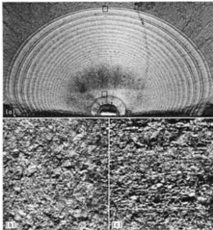
Fig. 54 Three views of a fatigue fracture in D6AC steel plate, showing beach marks. (a) Plate subjected to a series of varied loading cycles in the laboratory. The crack origin, at the bottom center, was at a starter notch formed by electrical discharge machining. (b) Area in lower square in (a), just above beach mark registering the first change in loading. (c) Area in upper square in (a), just ahead of the zone of final fast fracture. Both (b) and (c) contain faintly resolved, fine beach marks. (a) About 5 \times . (b) and (c) 60 \times . Source: Ref 124
