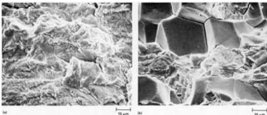
Fig. 80 Effect of hydrogen on the fatigue fracture appearance of a grade X42 pipeline steel. (a) Tested in dry nitrogen gas at a stress intensity range of \Delta K = 20 \text{ MPa } \sqrt{m} (18 ksi \sqrt{in} ), a load ratio of R = 0.1 , and a cyclic frequency of 5 Hz. (b) Tested in dry hydrogen gas at a stress intensity range of \Delta K = 10 \text{ MPa } \sqrt{m} (9 ksi \sqrt{in} ), a load ratio of R = 0.1 , and a cyclic frequency of 1 Hz. Both room-temperature fatigue tests resulted in a fatigue crack growth rate of approximately 2 \times 10^{-4} \text{ mm/cycle} . The fatigue fracture in nitrogen exhibited principally a serrated transgranular fracture, along with occasional bands of intergranular decohesion (not shown); however the fracture in hydrogen exhibited fewer regions of serrated fracture and more bands of intergranular decohesion. Source: Ref 218
