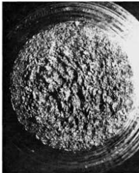
Fig. 426 Tension-overload fracture in a notched specimen of AISI 4340 steel, heat treated to a hardness of 27 HRC and tested at -40 °C (-40 °F), showing a completely fibrous surface. See Fig. 427 and 428 for fractures in similar specimens tested at different temperatures. 17×
