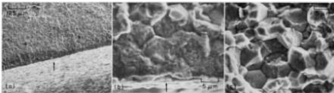
Fig. 102 Fracture caused by a portion of a pre-existing intergranular stress-corrosion crack that was not removed in reworking. The part was made of AISI 4340 steel that was heat treated to a tensile strength of 1790 to 1930 MPa (260 to 280 ksi). (a) and (b) Remains of an old crack along the edge of the surface of the part (arrows); note dark zone in (a) and extensively corroded separated grain facets in (b). (c) Clean intergranular portion of crack surface that formed at the time of final fracture
