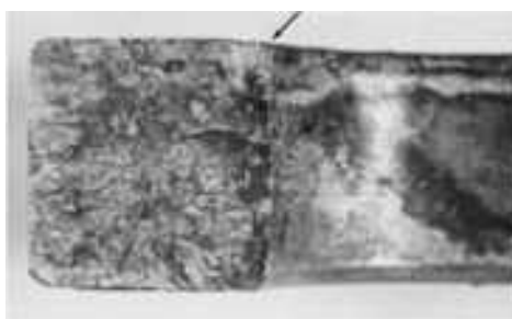
Fig. 1081 Fracture surface outboard of the bolthole in the lug at left in Fig. 1078. Here, as in Fig. 1079, the entire surface is typical of stress-corrosion cracking. Origin is at arrow (upper right corner of surface). 4×
