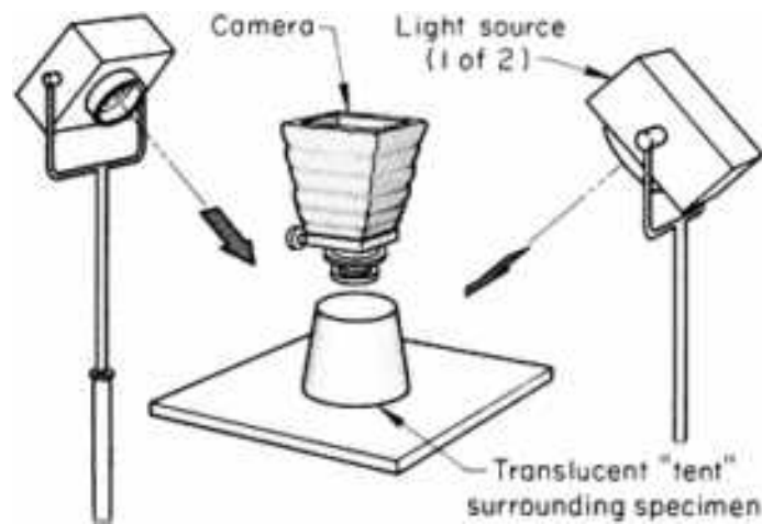
Fig. 18 Tent lighting used in photographing highly reflective parts
