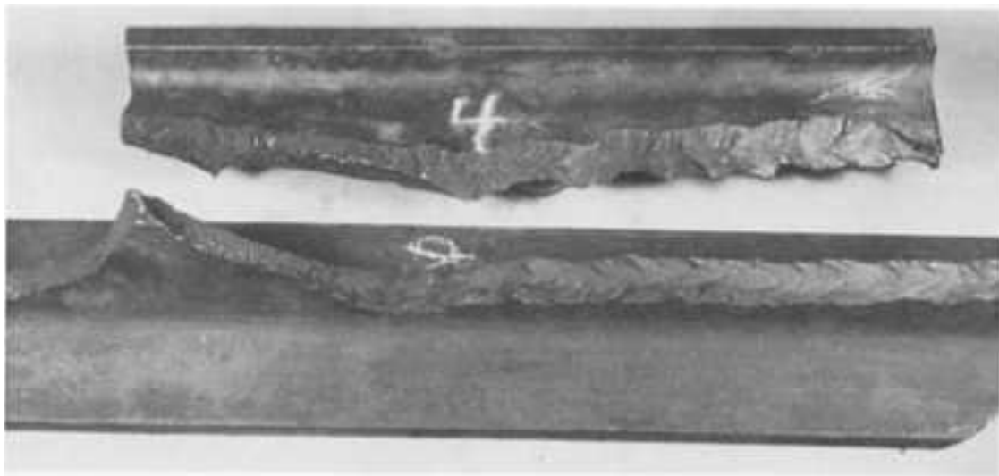
Fig. 39 Classic appearance of chevrons on a brittle fracture of a steel railroad rail. The fracture origin is not on the section shown.
