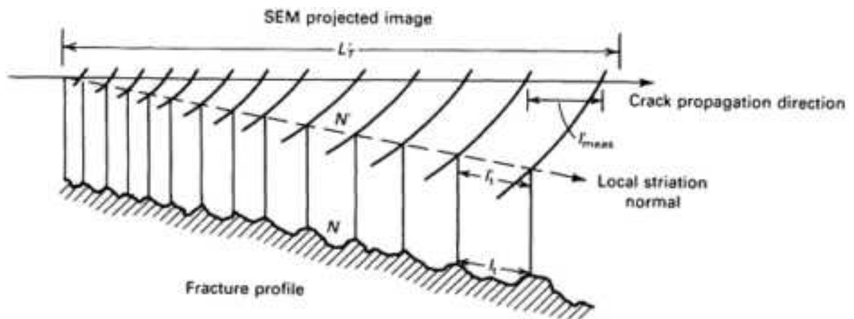
Fig. 18 Relationship of fatigue striation spacings to their projected images. L'_T : test line length; N : number of striations; l_t : true striation spacing; l'_{meas} : measured striation spacing in crack propagation direction. Primes indicate quantities in projection planes.
