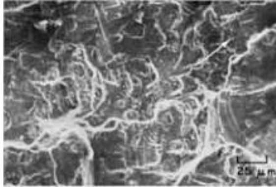
Fig. 1029 A typical region in an area A of Fig. 1027. Fatigue striations that are nearly vertical (arrow) are faintly visible. These were found to be parallel to the flaw (B-B in Fig. 1027) in both A areas in Fig. 1027. Scattered dimples are evident in locations adjacent to the fatigue striations. See also Fig. 1030. SEM, 400×
