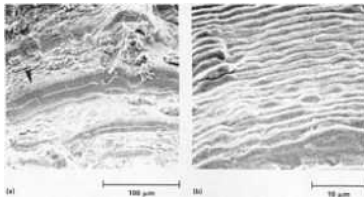
Fig. 84 Typical ridges and fatigue striations on the fracture surface of an annealed Incoloy 800 specimen tested in a sulfidizing atmosphere in the 316 - to 427 - \text{°C} ( 600 - to 800 - \text{°F} ) temperature range. (b) Higher-magnification fractograph of the area indicated by arrow in (a). Note the width of the smooth stretched areas at the ridges. Source: Ref 228
