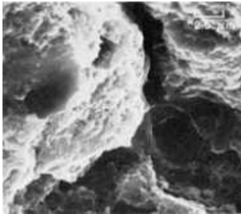
Fig. 1017 Enlarged view of the fracture-surface area in the rectangle in Fig. 1016. The higher magnification here makes it possible to observed the fine size of the dimples, which in general is less than half a micron. This is remarkable uniformity of size in a fracture surface as rough as this one. SEM, 4000×
