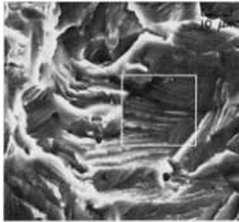
Fig. 1025 View of the fracture surface in Fig. 1024 that is very similar to the view of the low-cycle fracture surface in Fig. 1023. It is believed that the steplike formations resulted from a slip mechanism. Secondary cracks are not visible. See also Fig. 1026. SEM, 1000×
