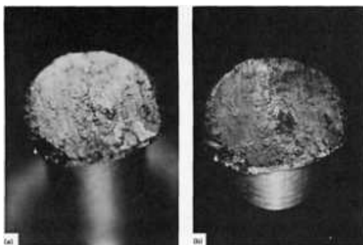
Fig. 4 Photographs of a fractured valve stem. (a) Conventional photography. (b) Scanning light photography. Both 10×. Courtesy of Irvine Optical Corporation.
