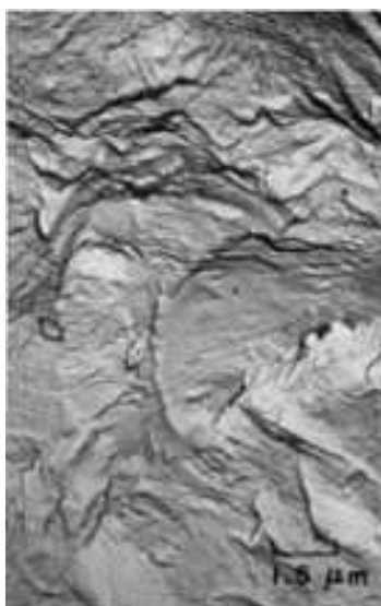
Fig. 1197 TEM p-c replica of an area at the fatigue-crack nucleus at A in the fracture surface in Fig. 1196, showing "brittle" fatigue striations (such as at the arrow at left center). 6500×
