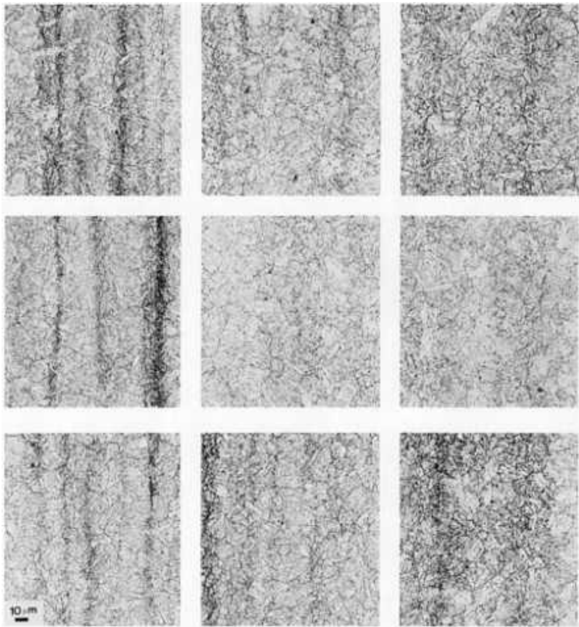
Fig. 99 Microstructures of AISI 4140 steel with 0.004% P (left column), 0.013% P (center column), and 0.022% P (right column). Specimens were etched with the ethereal-picral etchant described in Ref 442 (top row) and Ref 444 (middle row) and with saturated aqueous picric acid plus a wetting agent (bottom row). All 425×
