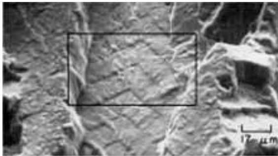
Fig. 1044 Corrosion-fatigue fracture in a specimen of aluminum alloy 7075-T6 tested in distilled water. Surface exhibits fatigue striations. The unusual sharp angle in the striations defines the location of a nearly vertical grain boundary in the central grain. Area in rectangle is shown at higher magnification in Fig. 1045. SEM, 600×
