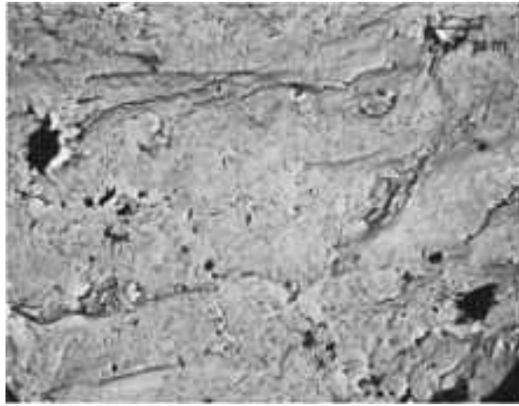
Fig. 714 TEM p-c replica of the fracture surface in Fig. 711, showing a region about 30 \mu\text{m} from the inner edge. This view shows generally flat fatigue patches that are separated by steps, but no fatigue striations are visible within the patches. 3750 \times
